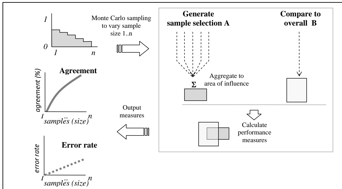
Figure 2. Illustration of Monte Carlo procedure to perform repeated random sampling of spatial data to create a selection A, to spatially aggregate this set and compare it with B, and to report performance measures as output.
